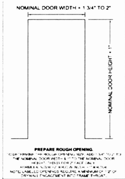
Drywall KD Hollow Metal Frame Nominal Door Width Plus 1 3/4" - 2" Nominal Door Height Plus 1"
